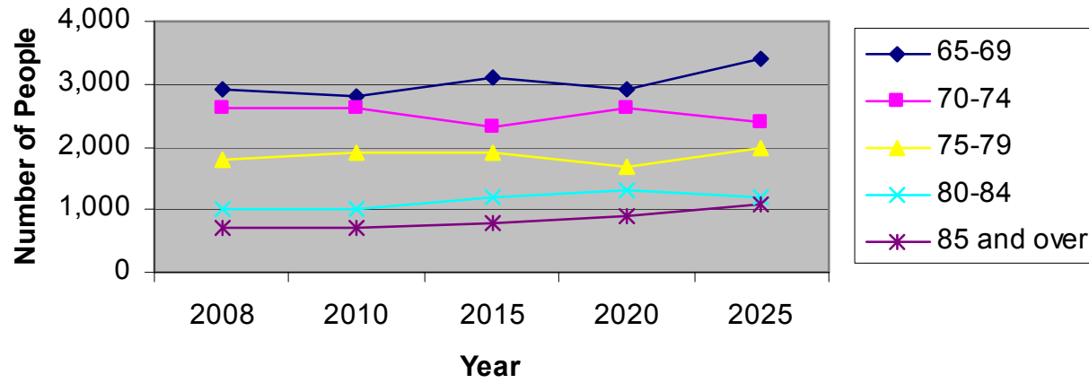
Populations projections of Males aged 65yrs+
