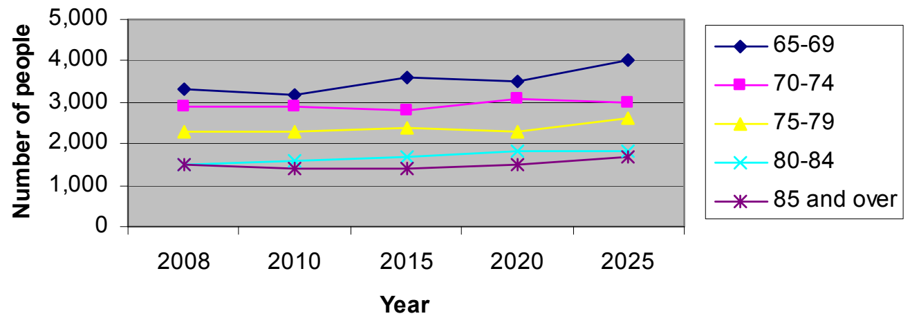
Population projections of Females aged 65yrs+
